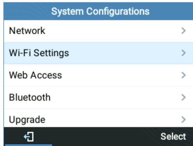
Figure 80: Wi-Fi feature
