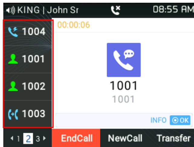
Figure 56: VPK Paging
