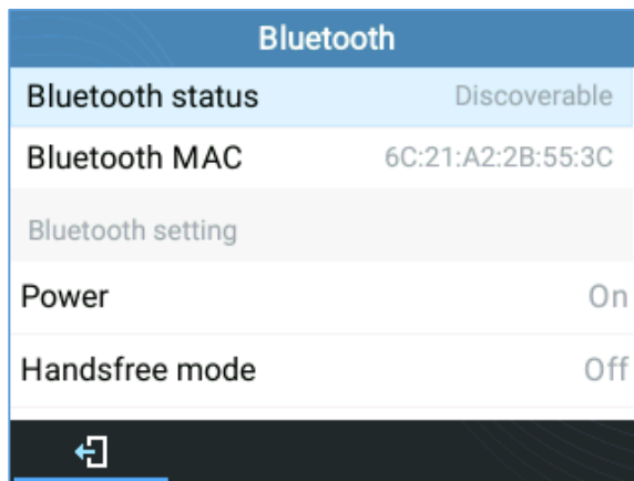
Figure 78: Bluetooth Status
