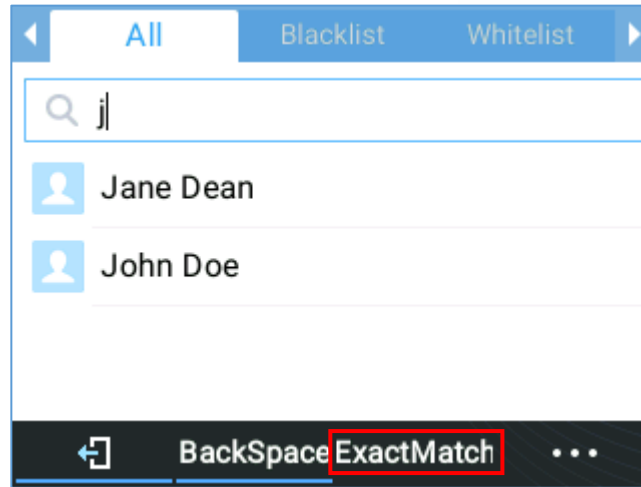
Figure 68: ExactMatch
