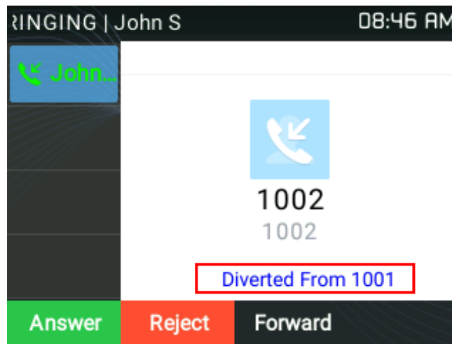
Figure 42: Diversion Information
