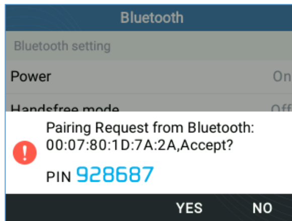
Figure 79: Pairing Request
