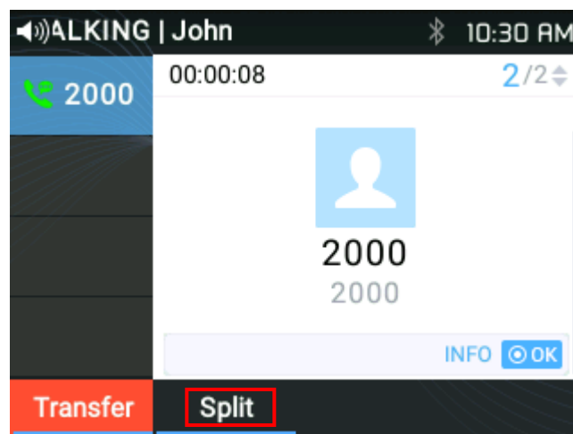
Figure 26: "Split" softkey
