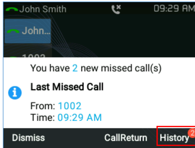
Figure 72: Missed Calls
