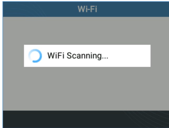
Figure 82: Wi-Fi Scanning
