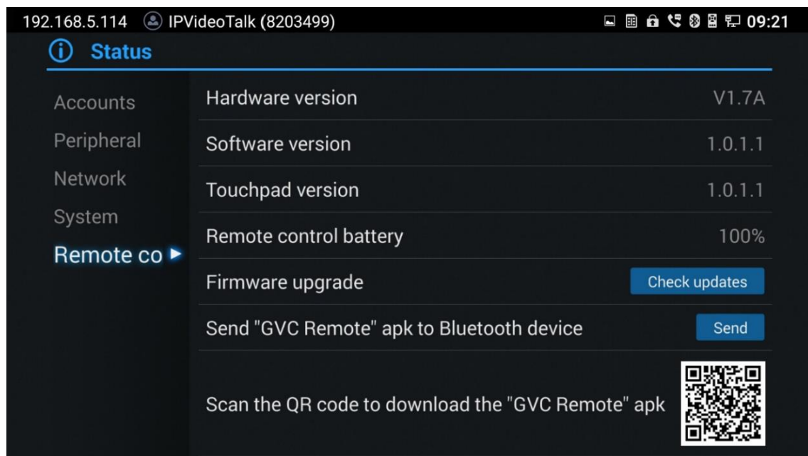
Figure 67: "GVC Remote" apk in GVC3210 LCD Menu → Settings → Status → Remote Control
