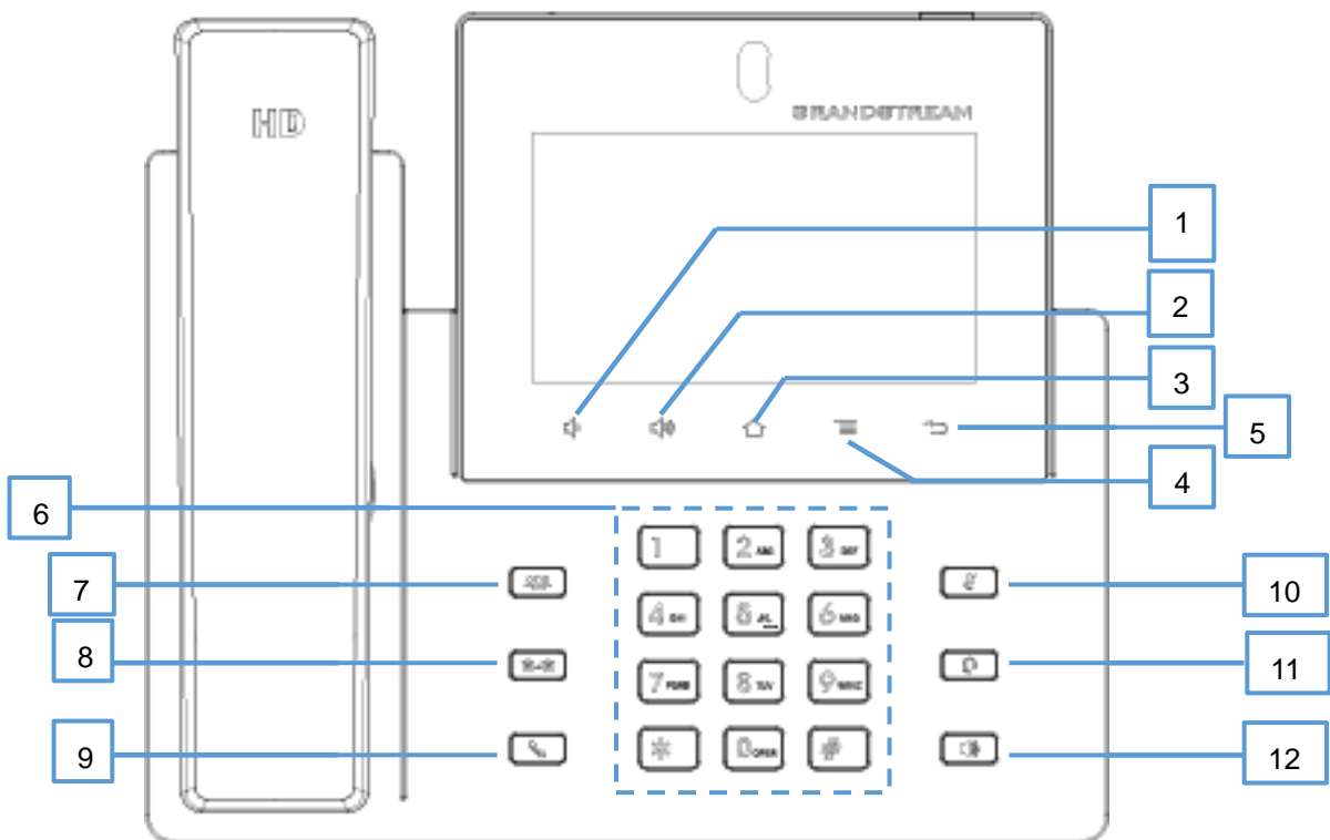
Figure 29: GXV3350 Keys
