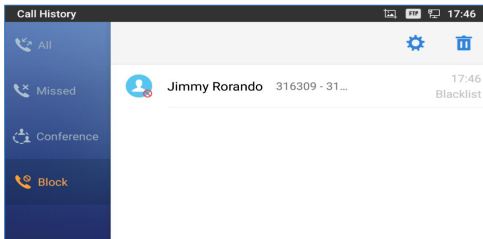
Figure 103: Block History
