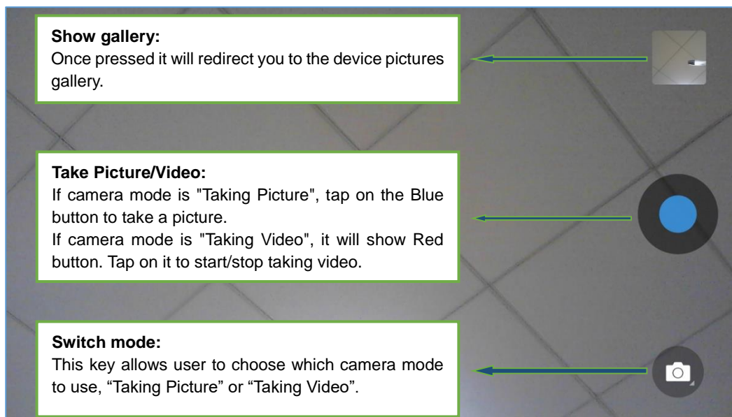
Figure 126: GXV3350 Camera
