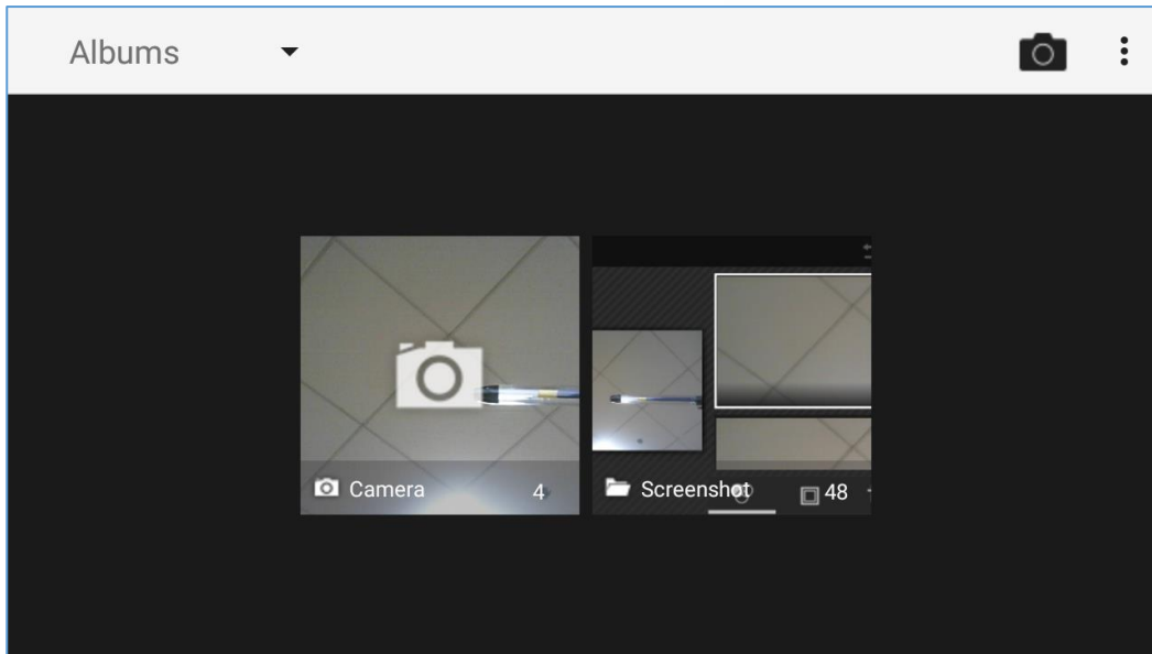
Figure 130: GXV3350 Gallery
