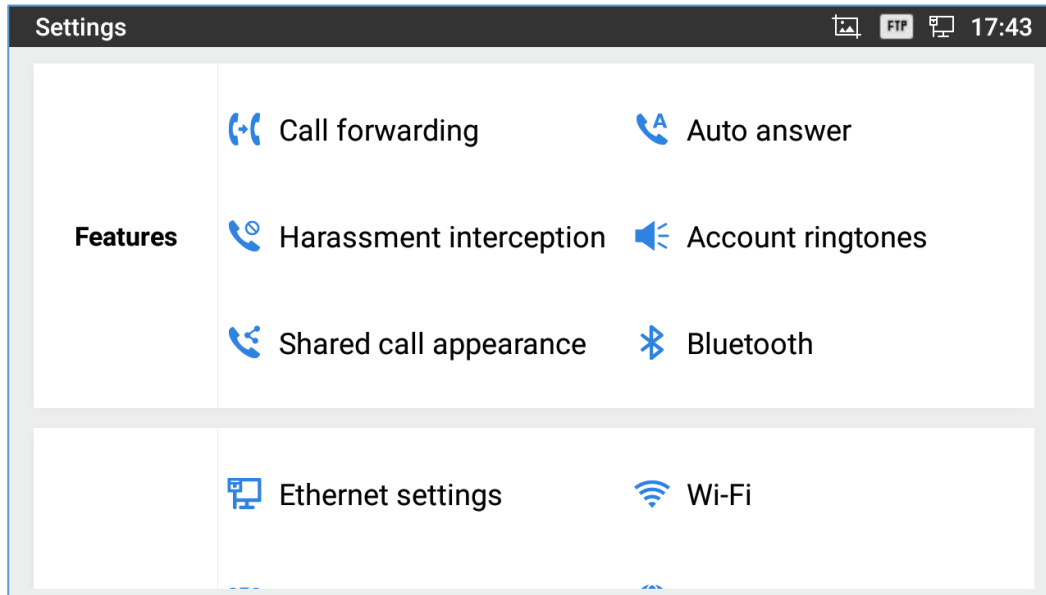
Figure 101: GXV3350 Settings
