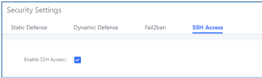
Figure 39: SSH Access
