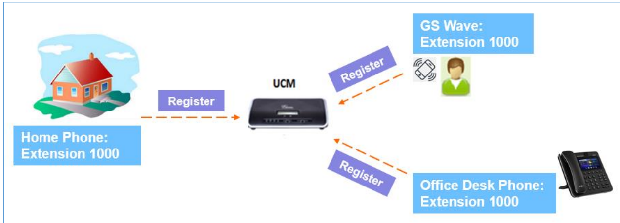
Figure 102: Multiple Registrations per Extension
